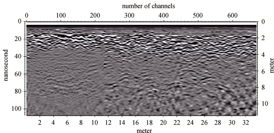
Fig. 6 Primary test result of geological structure from the second channel of LPR
