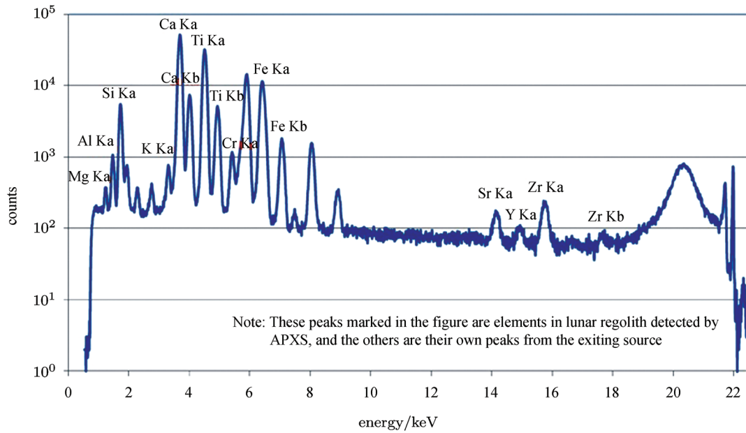
Fig. 7 EDS image of the lunar regolith detected by APXS in-situ in the orbit
