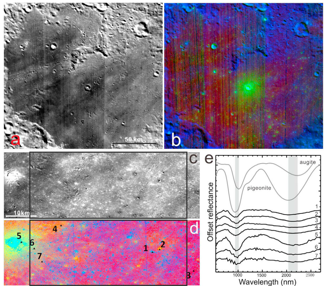
Figure 5. (a) M^3 750 nm reflectance mosaic of Von Kármán crater (stretch: 0.044–0.082). High albedo linear features oriented WSW-ESE are visible on the crater floor, and they can be traced back to Finsen crater in Figure 1b. The location of this subset and (b) is indicated in Figure 1b. (b) M^3 color composite of Von Kármán crater (same region as a). R = 2 \mu m band center (2,000–2,500); G = 2 \mu m band depth (0.04–0.17); B = reflectance at 1580 nm (0.085–0.15). Stretch values are indicated in brackets. LCP-bearing material appears in light blue, and HCP-bearing material appears green. Spectral parameters were calculated using the method described in Martinot et al. (2018). (c) MI 750 nm reflectance mosaic of the landing area. Relatively high albedo features are mostly associated with ejecta deposits of small fresh craters, and impact rays from the Finsen crater, whereas low albedo features are mostly associated with mare basalts and ejecta deposits of large craters. The landing area is indicated as a black rectangle, which is indicated in Figure 1d. (d) RGB composite of MI data. R: 750 nm/415 nm (1.797–1.925), G: 950 nm/750 nm (0.877–1.034), B: 415 nm/750 nm (0.515–0.564). Stretch values are indicated in brackets. The landing area is indicated as a black rectangle, which is indicated in Figure 1d. (e) Continuum-removed M^3 spectra of locations (1 to 7) in Figure 5d. Each spectrum corresponds to a single pixel. Spectra were processed with the method described in Martinot et al. (2018). A pigeonite (LCP) and an augite (HCP) spectrum from the RELAB database are displayed above the observed spectra for comparison (respective RELAB-ID: DL-CMP-008 and AG-TJM-010). The shaded areas represent the diversity of values of the 1 and 2 \mu m bands.
