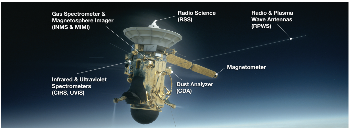
Eight of Cassini's science instruments are planned to be turned on during the final plunge, including the Ion and neutral Mass Spectrometer (INMS). Credit: NASA/JPL-Caltech
