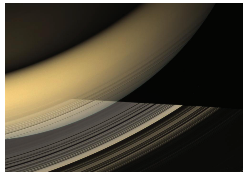
Shadowed Rings
