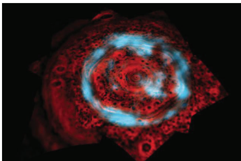
Above Saturn
