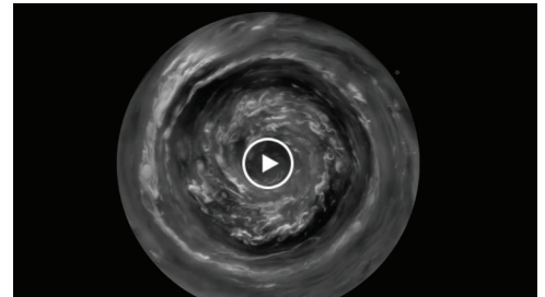
Saturn Hurricane
