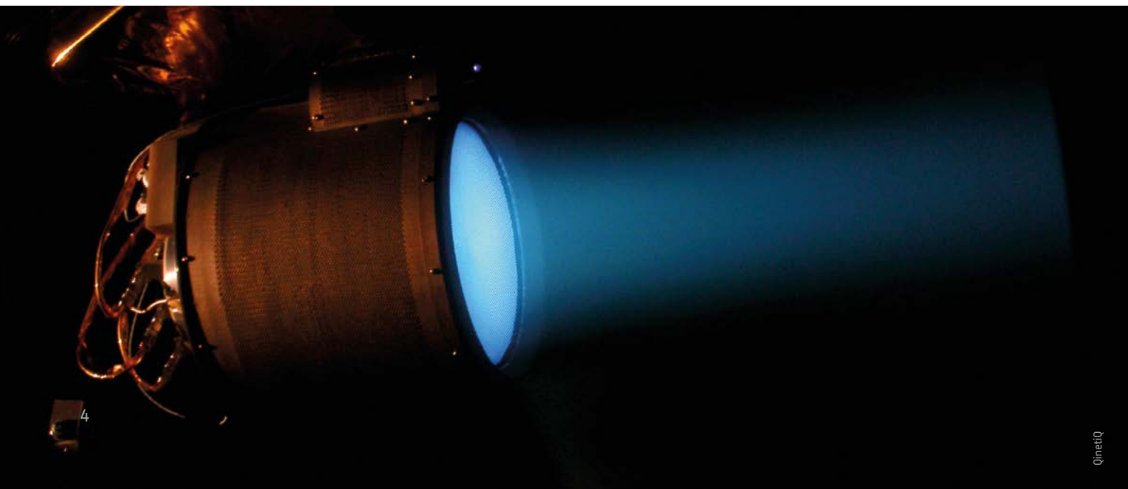
An ion thruster during a test firing. Four thrusters are installed on the Mercury Transfer Module
