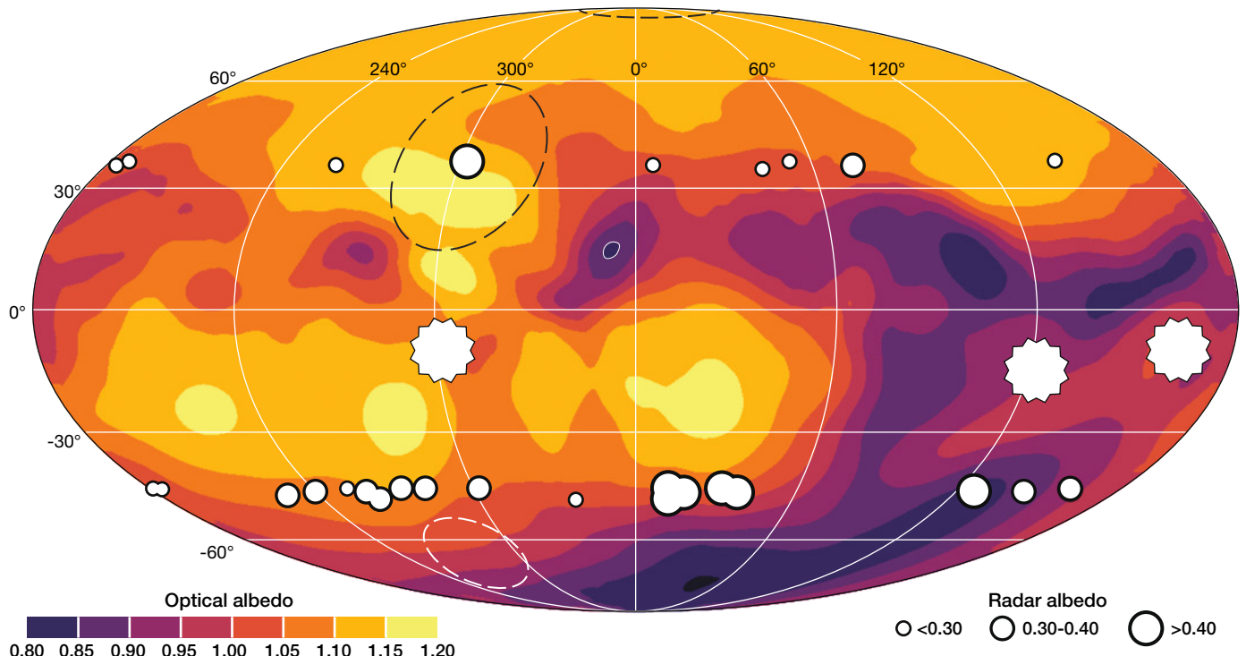
PSYCHE SPACECRAFT, ARIZONA STATE UNIVERSITY; ALBEDO MAP OF PSYCHE, M. K. SHEPARD ET AL. / PLANETARY SCIENCE JOURNAL 2021
