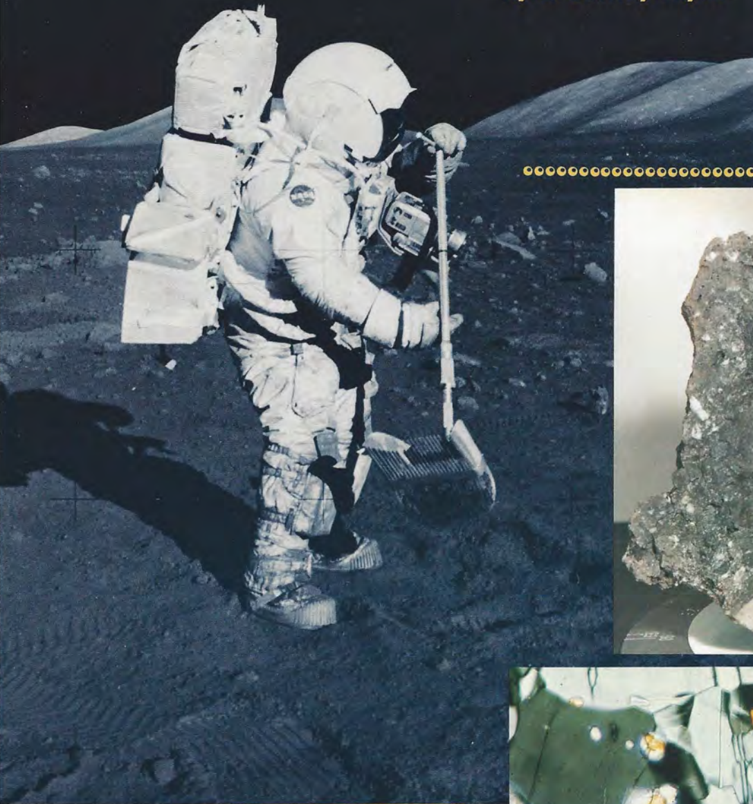
ABOVE: Scientist-astronaut Harrison H. Schmitt collects lunar rake samples at the Taurus-Littrow landing site during the Apollo 17 mission. His lunar rake collected discrete samples of rocks and rock chips ranging in size from one-half inch (1.3 cm) to one inch (2.5 cm).
