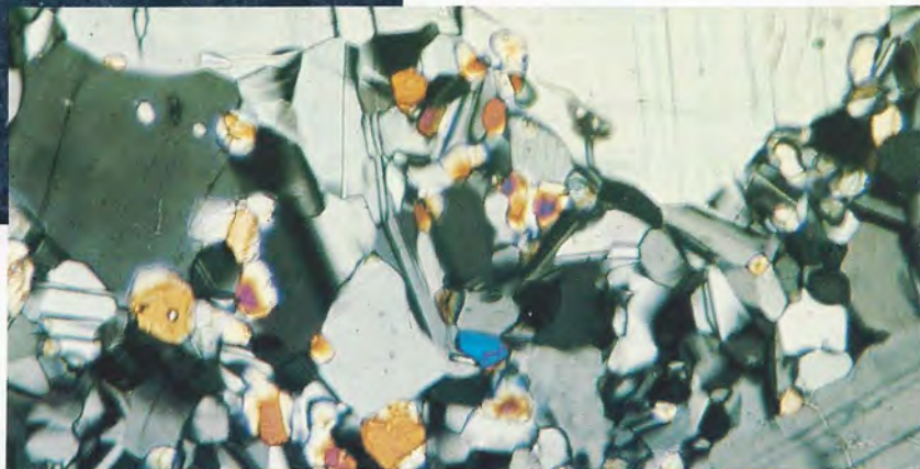
ABOVE: This microscopic view (1.5 millimeters across) of a mare basalt was made by shining polarized light through a wafer of rock 30 micrometers thick. The shapes and sizes of the minerals indicate that the rock crystallized in a lava flow. Pyroxene appears as orange and blue, the gray is feldspar.
